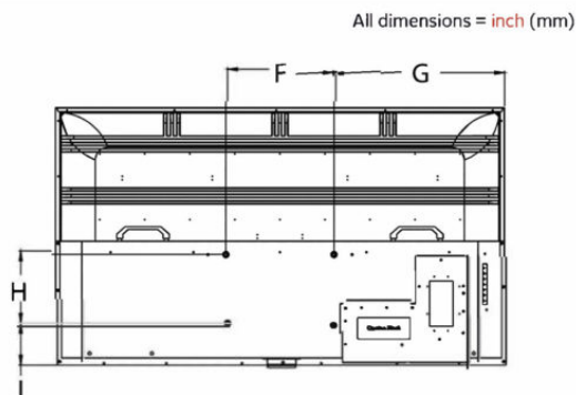
BACK VIEW
