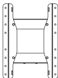
VESA 300x200 VESA 300x300 ADAPTOR DETAIL
