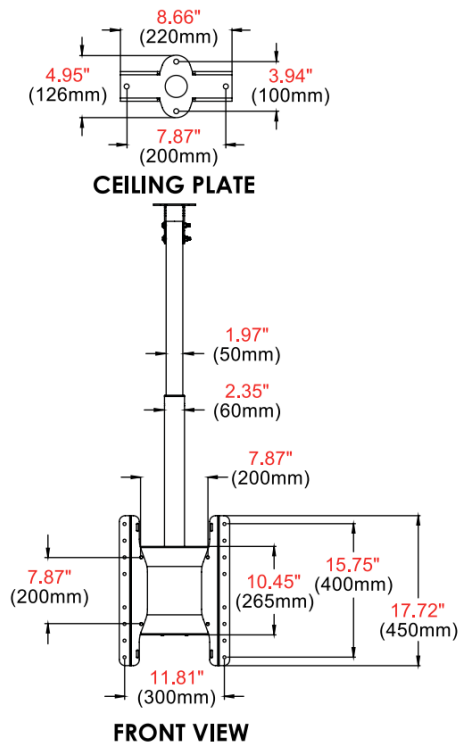
VESA 200x100 VESA 200x200 ADAPTOR DETAIL
