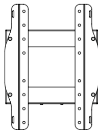
VESA 200x100 VESA 200x200 ADAPTOR DETAIL
