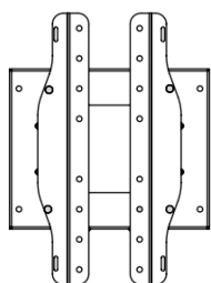
VESA 100x100 ADAPTOR DETAIL
